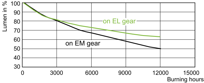
CDM-T 70W Lumen Maintenance /942
