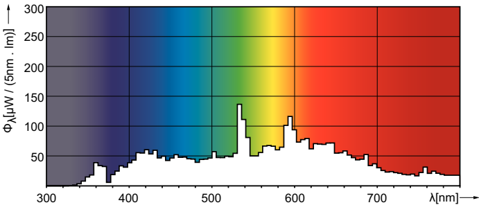
MASTERColour CDM-T 70W, 150W /942
