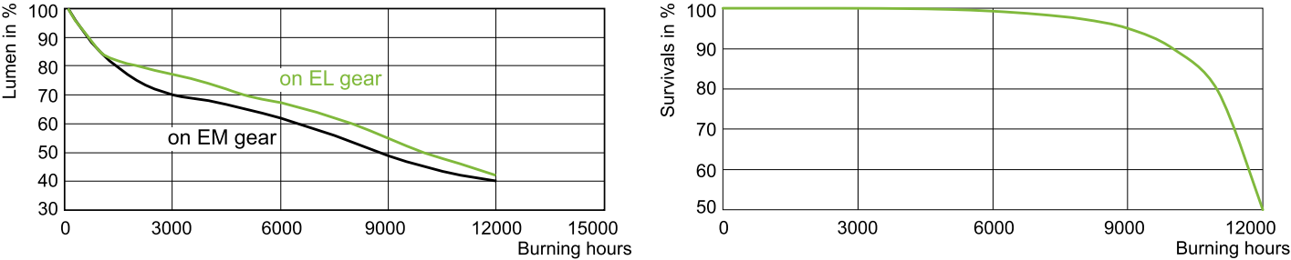
CDM-T 35W Lumen Maintenance /830
