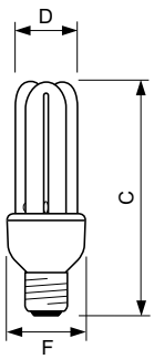
Econ Genie ErP NG 14W/865 E27 220-240V
